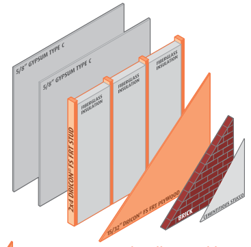
Two-Hour Wood Wall Assembly (2hr interior and 1hr exterior face)
